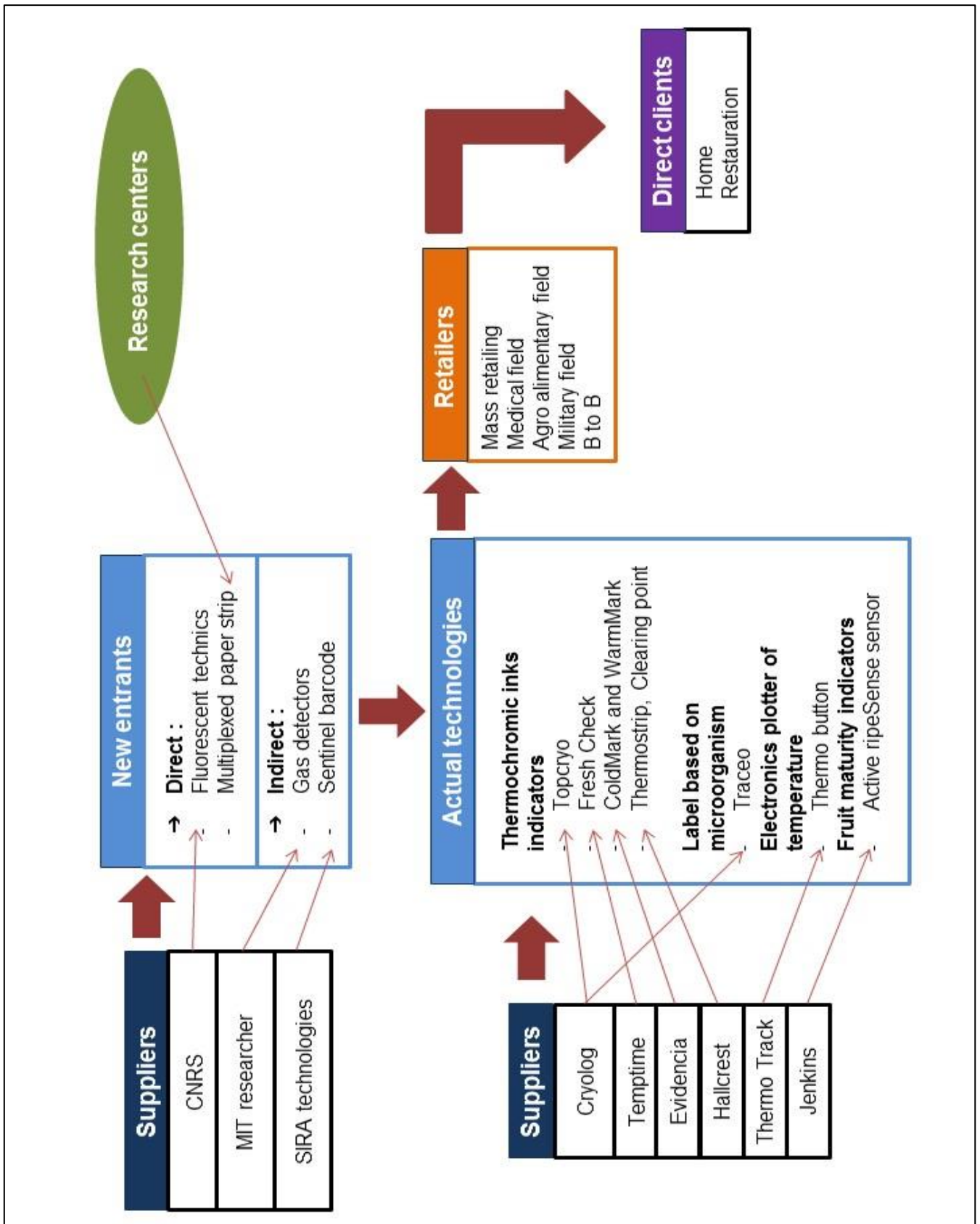
Scheme 15: Porter diagram
